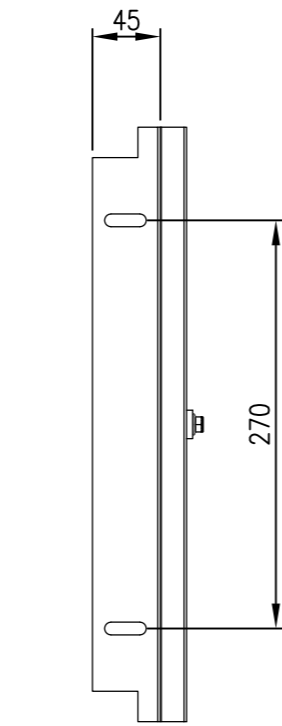
RIGHT SIDE VERTICAL FRAME
