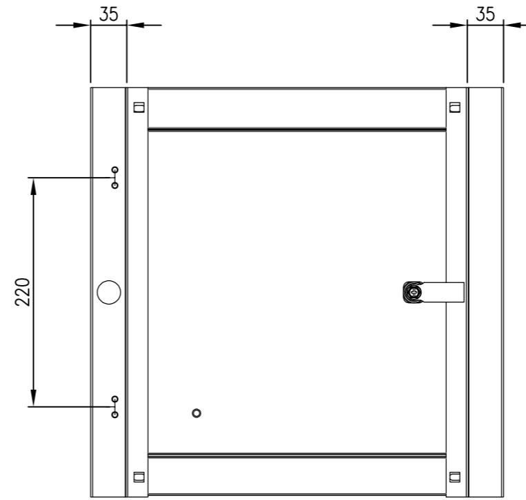
REAR VIEW
