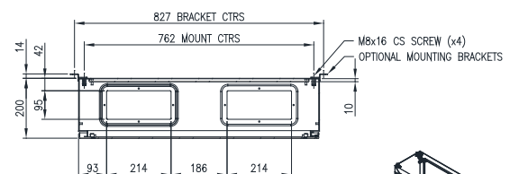
SECTION AW-AW
